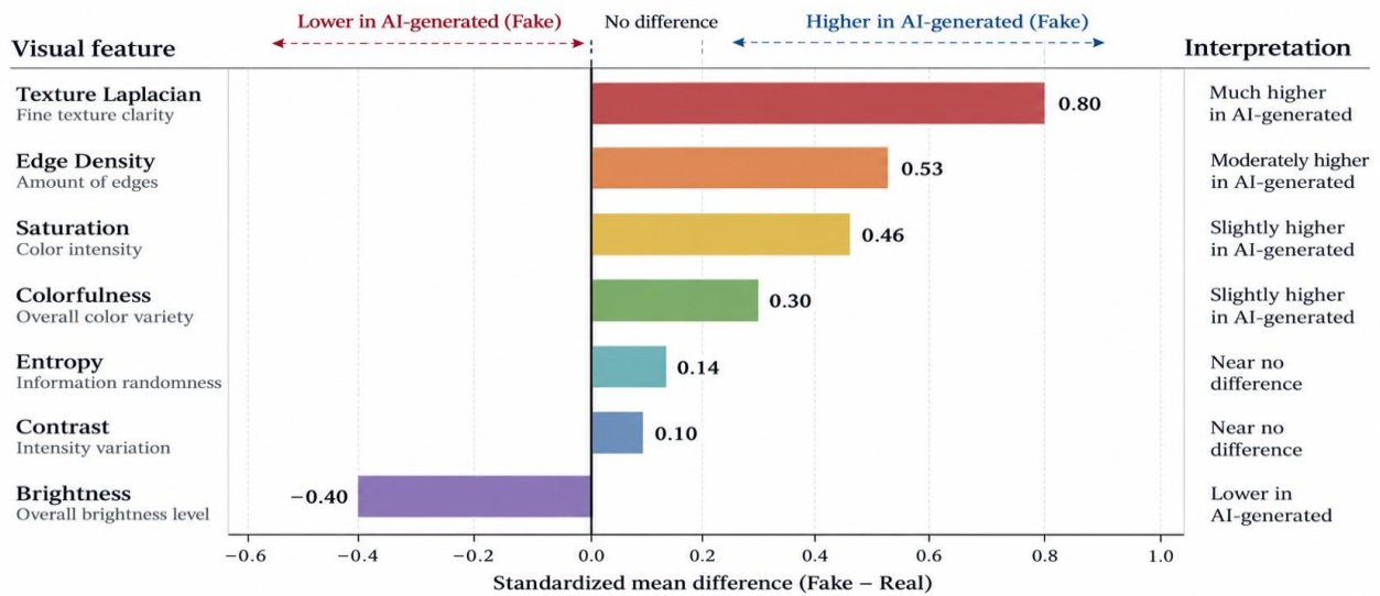
FIGURE 3. Visual feature differences between real and AI-generated images.
